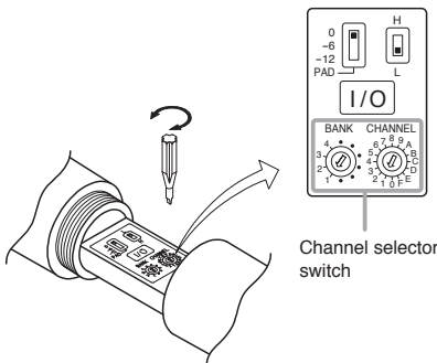
Pad switch
