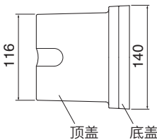
[侧面]
