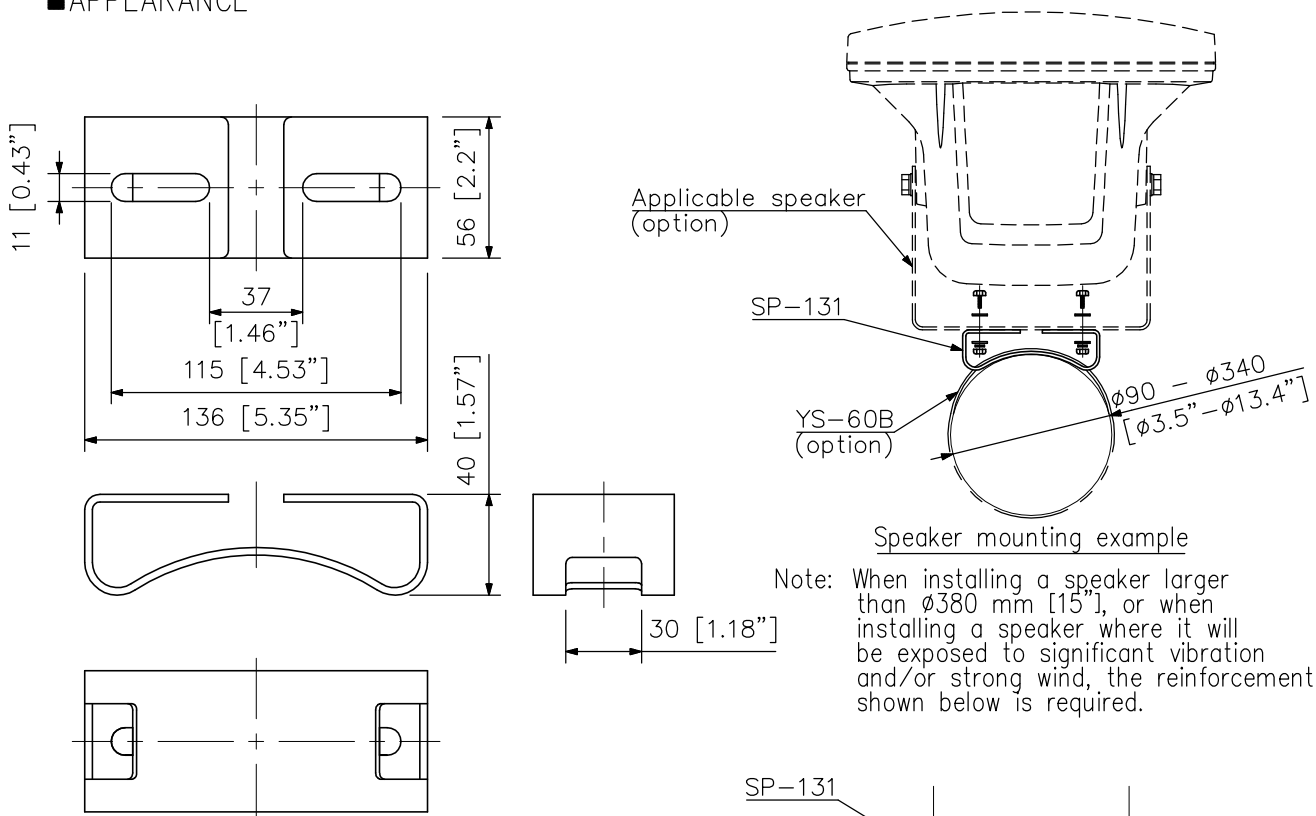
Mounting bracket (t3.0)
