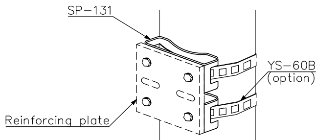
Example of mounting reinforcement
