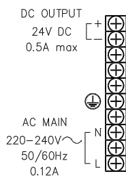
Terminal block
