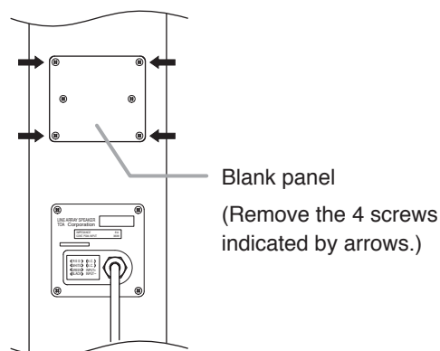
SR-S4LWP/S4SWP Rear panel
