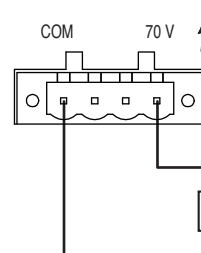
Speaker output terminal
