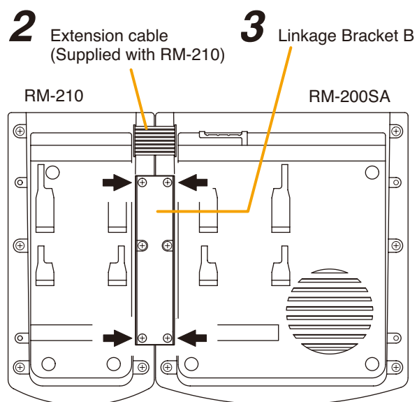
[Bottom side]
