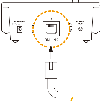
RM-200SA rear
