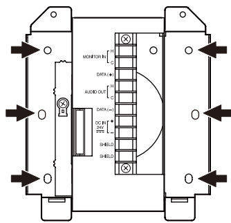
Wall mount bracket unit (supplied with the RM-200SF)
