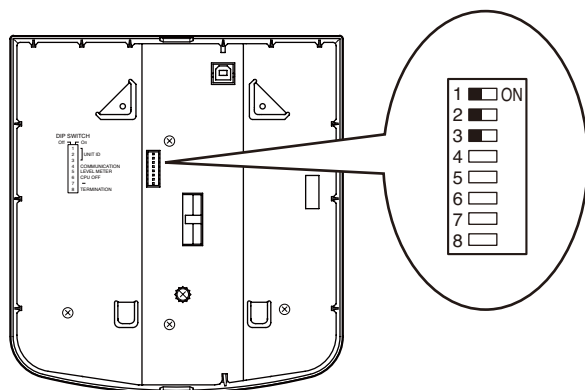
RM-200SF bottom
