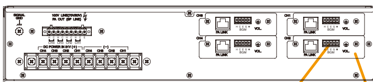
BGM input PA link/BGM input board
