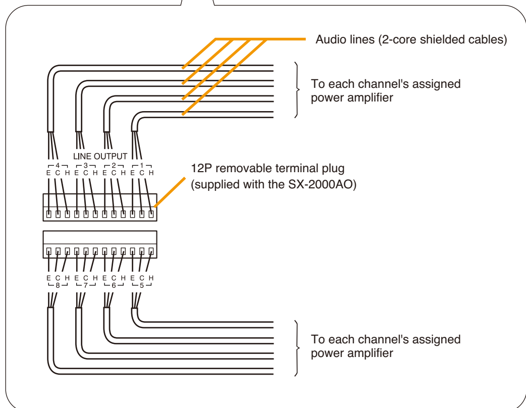
Audio output terminals
