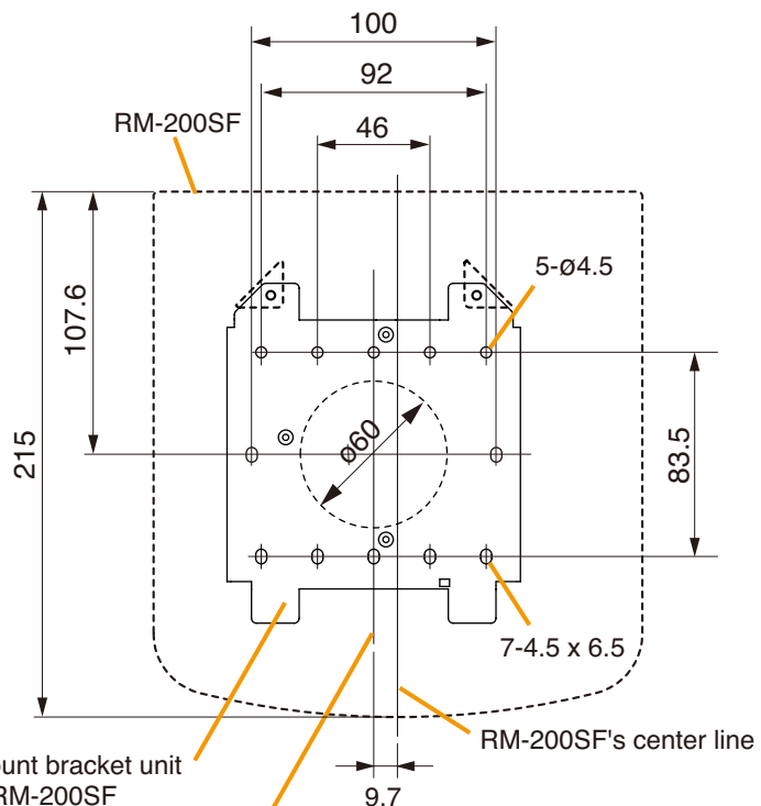
Wall mount bracket unit's center line
