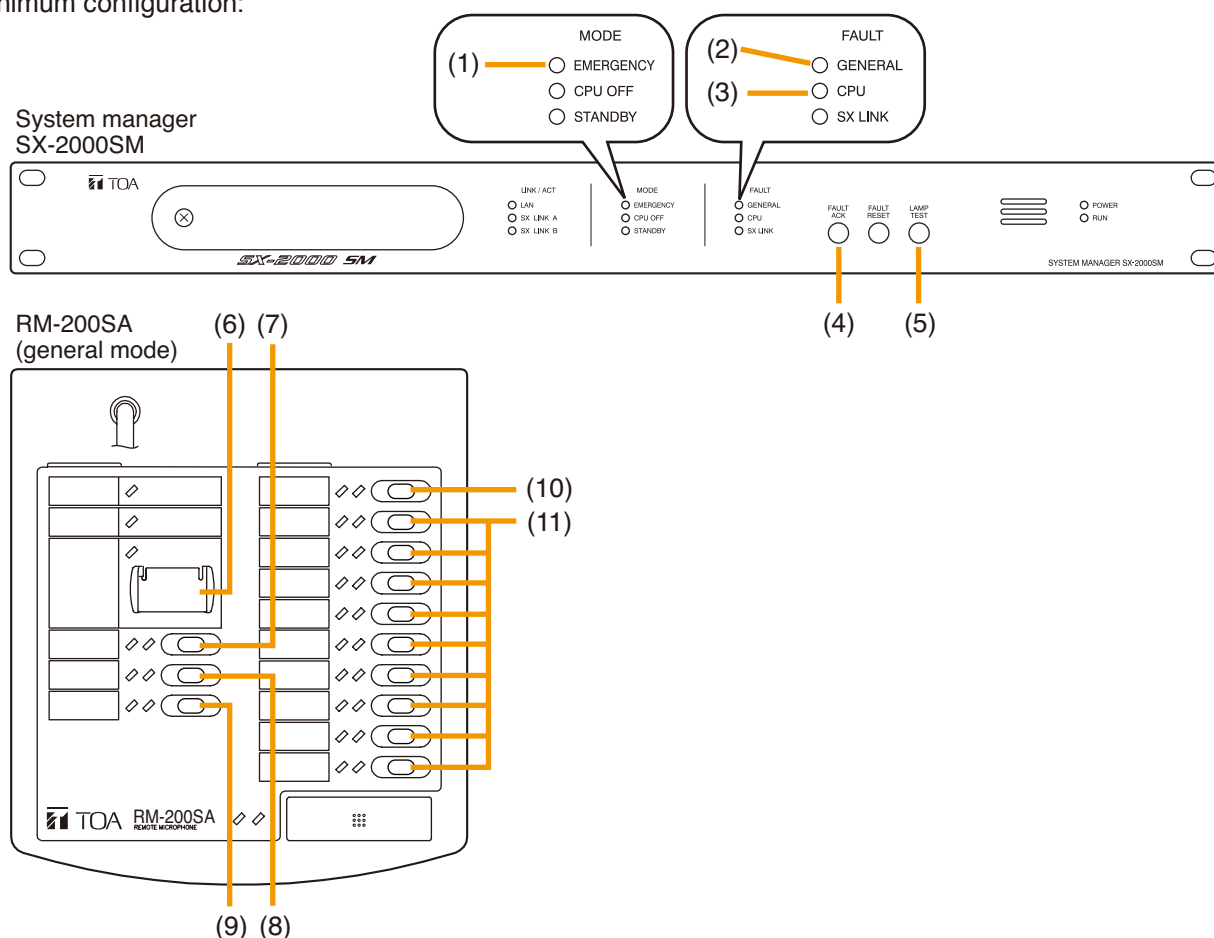
Figure 1: Minimum configuration for mandatory indications and controls
