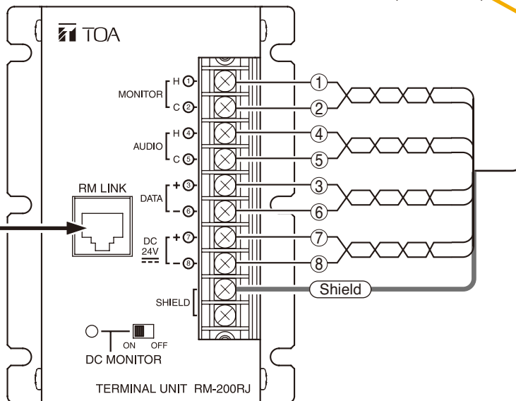
RM-200RJ
