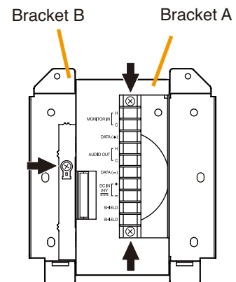
Wall mount bracket unit (supplied with the RM-200SF)
