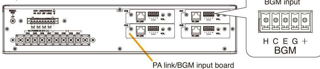
Amplifier's rear
