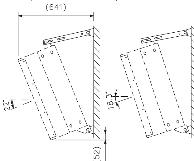
ES-0871 mounting example (scale: 1/20)
