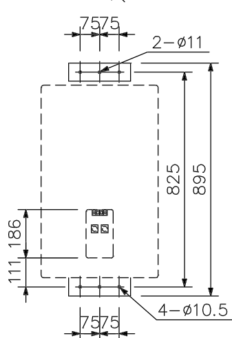
Dimension for mounting ES-0871 speaker (scale: 1/20)
