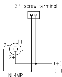
Wiring Diagram
