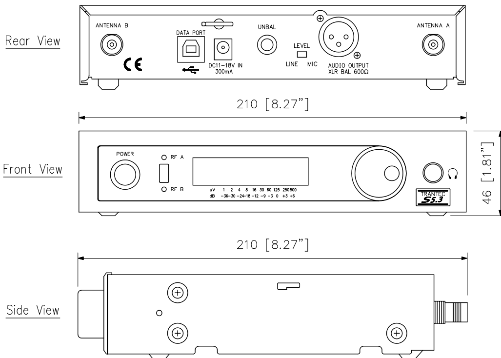
Wireless tuner
