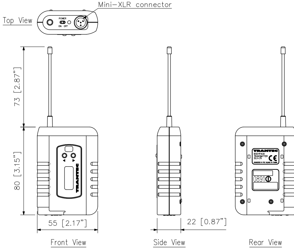
Wireless transmitter
