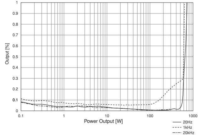
Distortion (8Ω)
