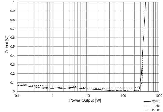
Distortion (8Ω)
