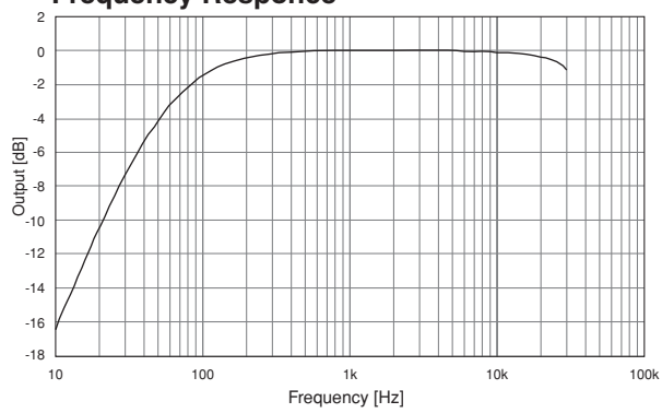
Frequency Response
