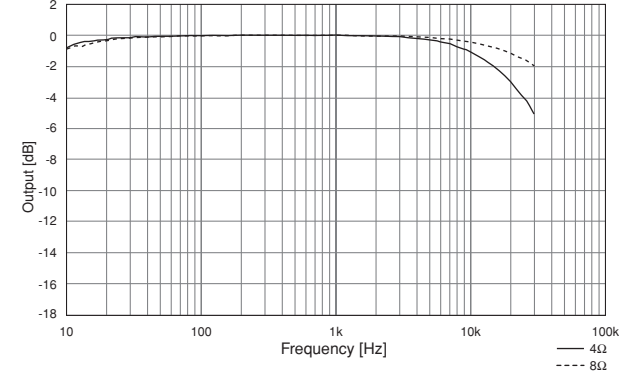
Frequency Responce
