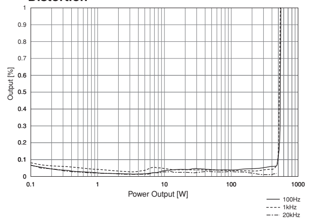
Distortion
