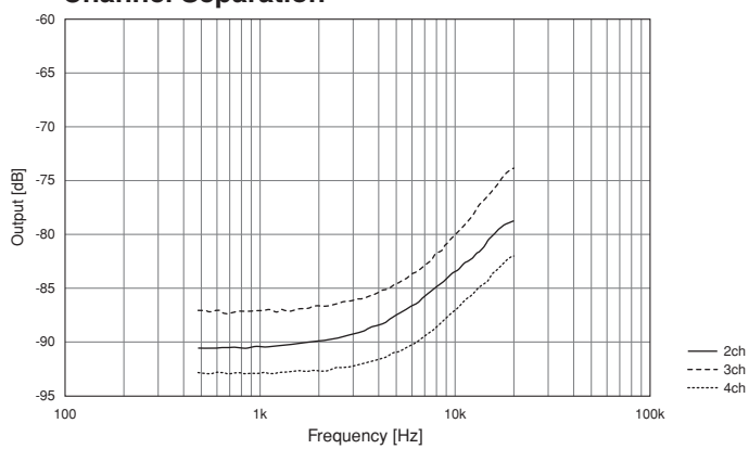
Channel Separation
