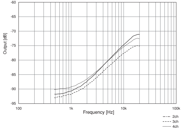
Channel Separation
