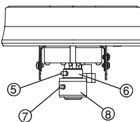
Bottom view without inner cover
