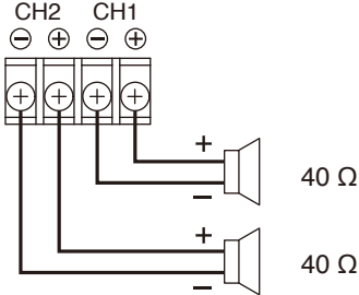
Speaker output terminals
