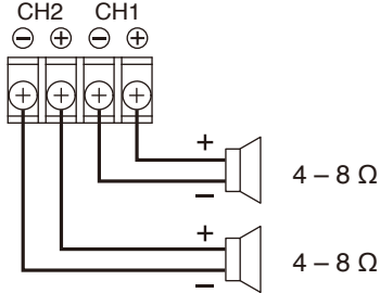
Speaker output terminals
