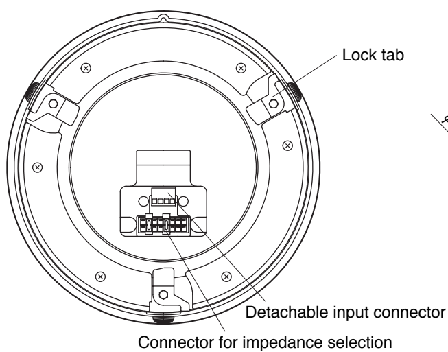
[Installation Example]
